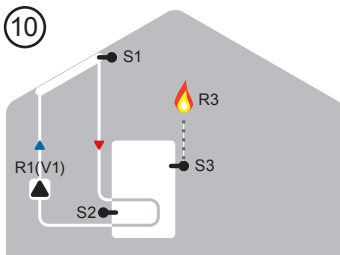
Solar + Thermostat
