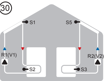
2 x Solar
