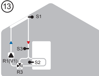
Solar + Bypass
